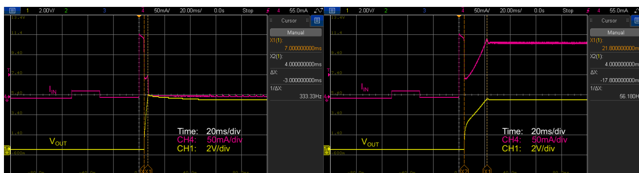
Figure 32. Si3406-ISO-FB EVB, 5 V, Class 2 Output Voltage Soft-Start at Low Load (Left) and Heavy Load (Right) Conditions
