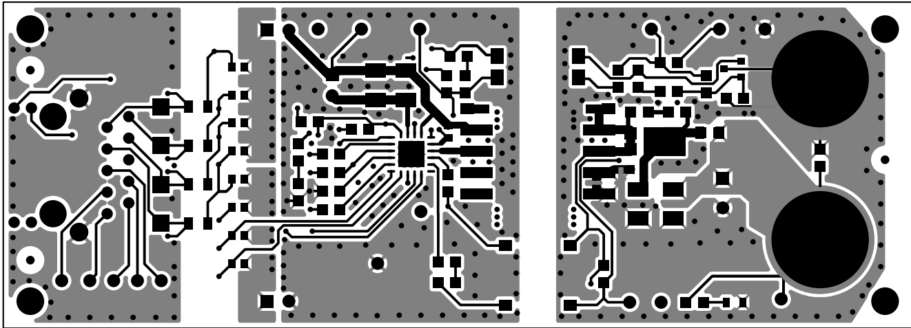
Figure 64. Top Layer
