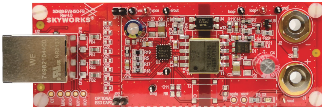
Figure 1. Si3406 Isolated Flyback Evaluation Board
