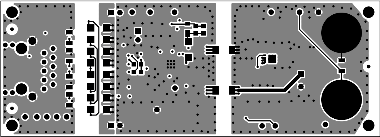
Figure 67. Bottom Layer
