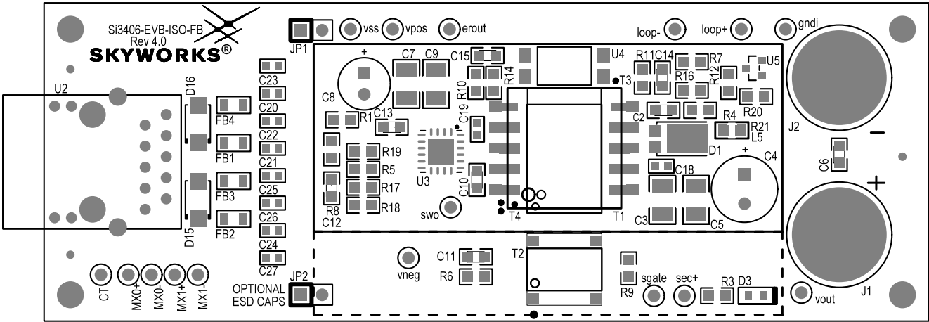
Figure 63. Top Silkscreen
